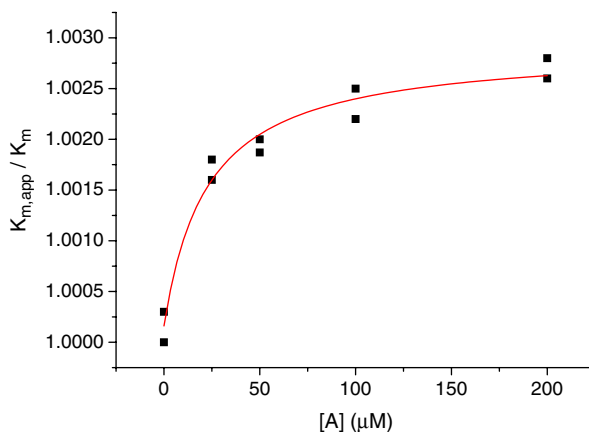
Fig. 3 Nonlinear least-squares curve fittings of the K_{m, app}/K_m value for the BChE-catalyzed hydrolysis of BTCh vs. activator 1 concentration ( [A] ) plot against Eq. 3. The parameters of the fit were \alpha K_A = 23 \pm 6 \mu\text{M} and \alpha = 1.0029 \pm 0.0002 ( R^2 = 0.9745 )
